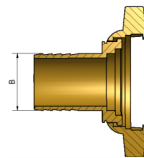
FEMMINA CON ALETTE E PORTAGOMMA FEMALE WITH WINGS AND INSERT
