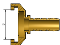
CON PORTAGOMMA E COLLARINO WITH INSERT AND COLLAR
